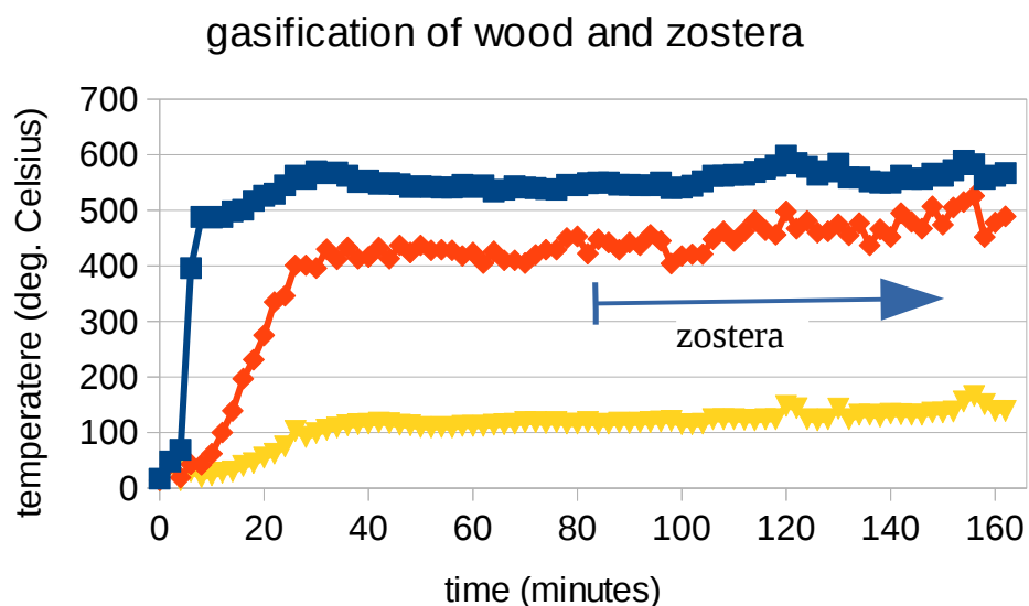
Figure 3: temperatures in the gasifier during the gasification of wood pellets (first 80 minutes) and zoster marina .
